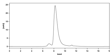
Bioactivity
