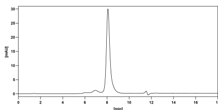
SEC-HPLC detection for InVivoMAb Anti-Human IL10 (ABV0256).
